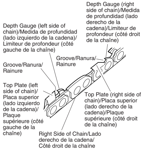
Figure 22 - Chain Part Locations
